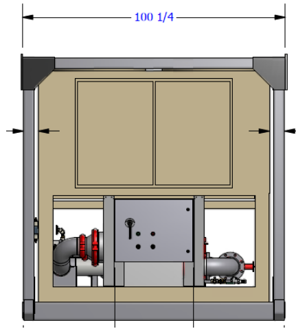
Control and Electrical Panels with Dimensional Data
