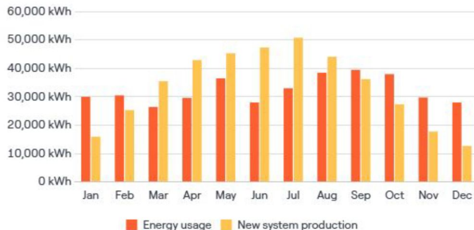
Monthly production (kWh)
